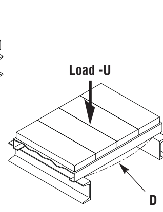
Figure 2c Uniform Load
